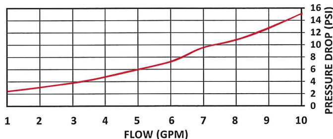
ICVN NOZZLE
